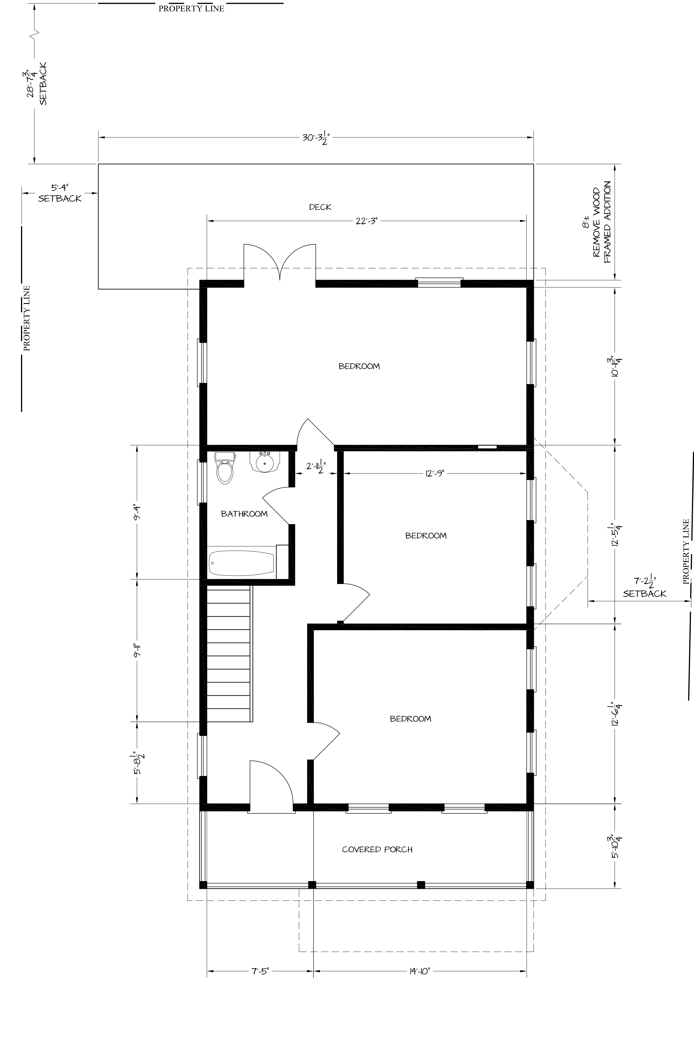
2ND FLOOR (EXISTING / DEMO) 1/4" = 1'-0"
