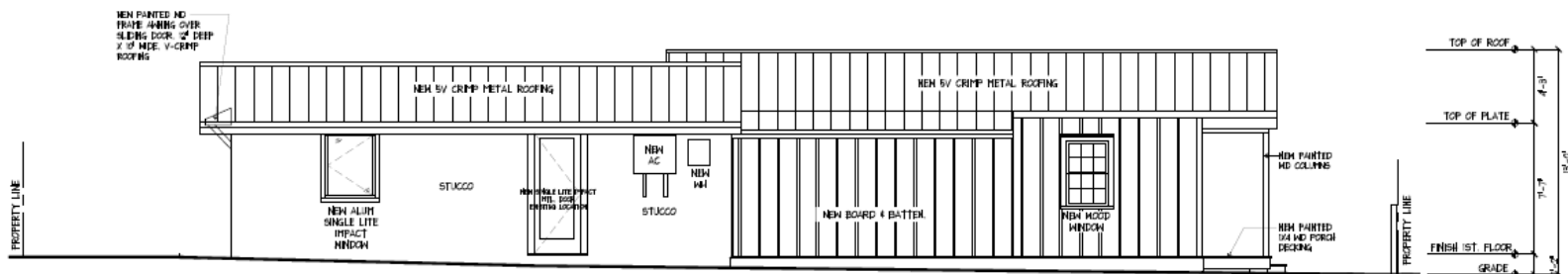
1 PROPOSED WEST ELEVATION
