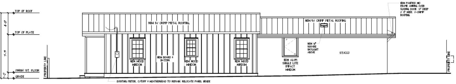
2 PROPOSED EAST ELEVATION
