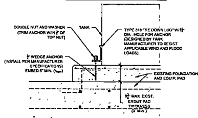
TYP. DETAIL - TANK ANCHOR
