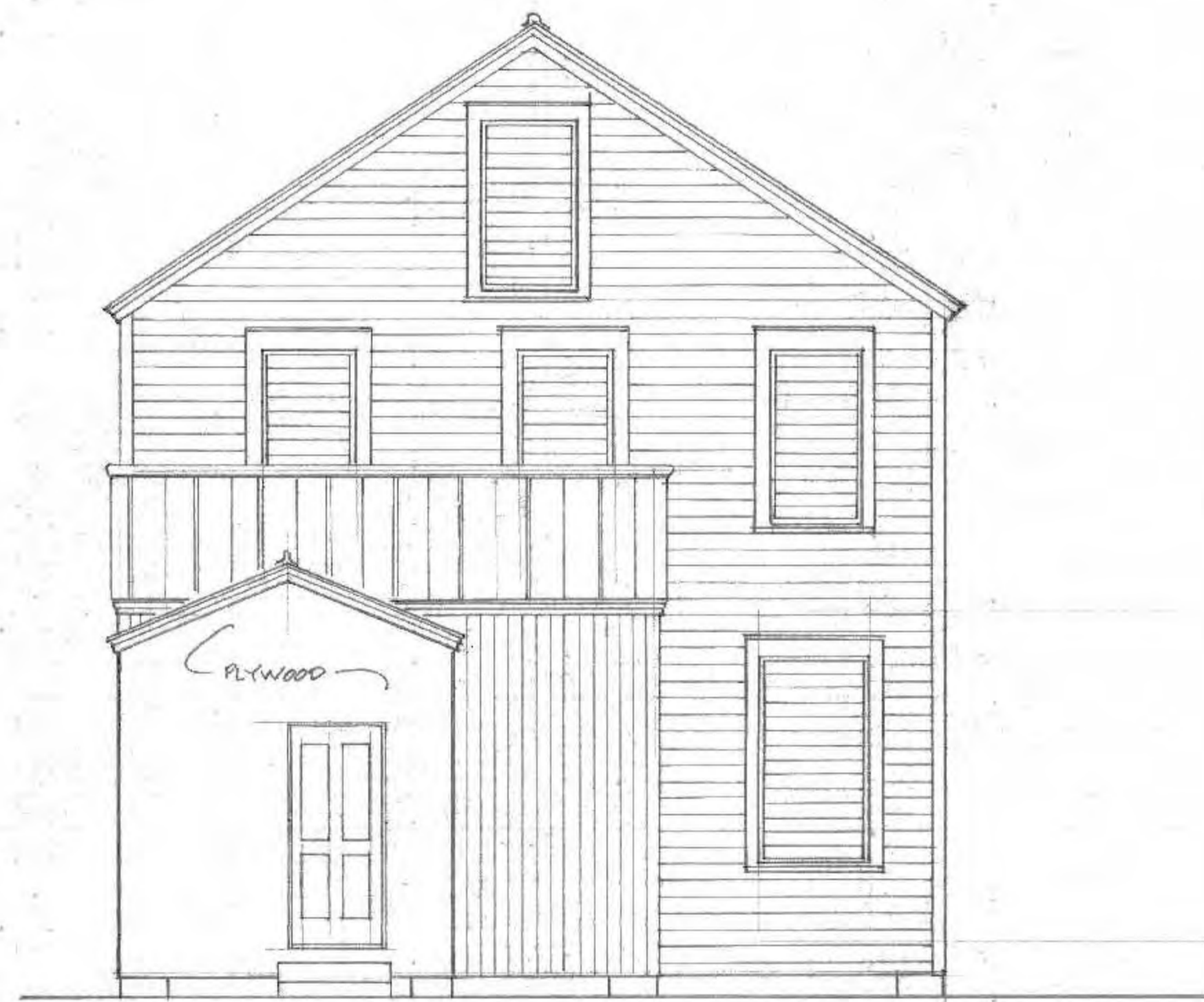
SOUTHEAST ELEVATION 1/4"=1'-0"
