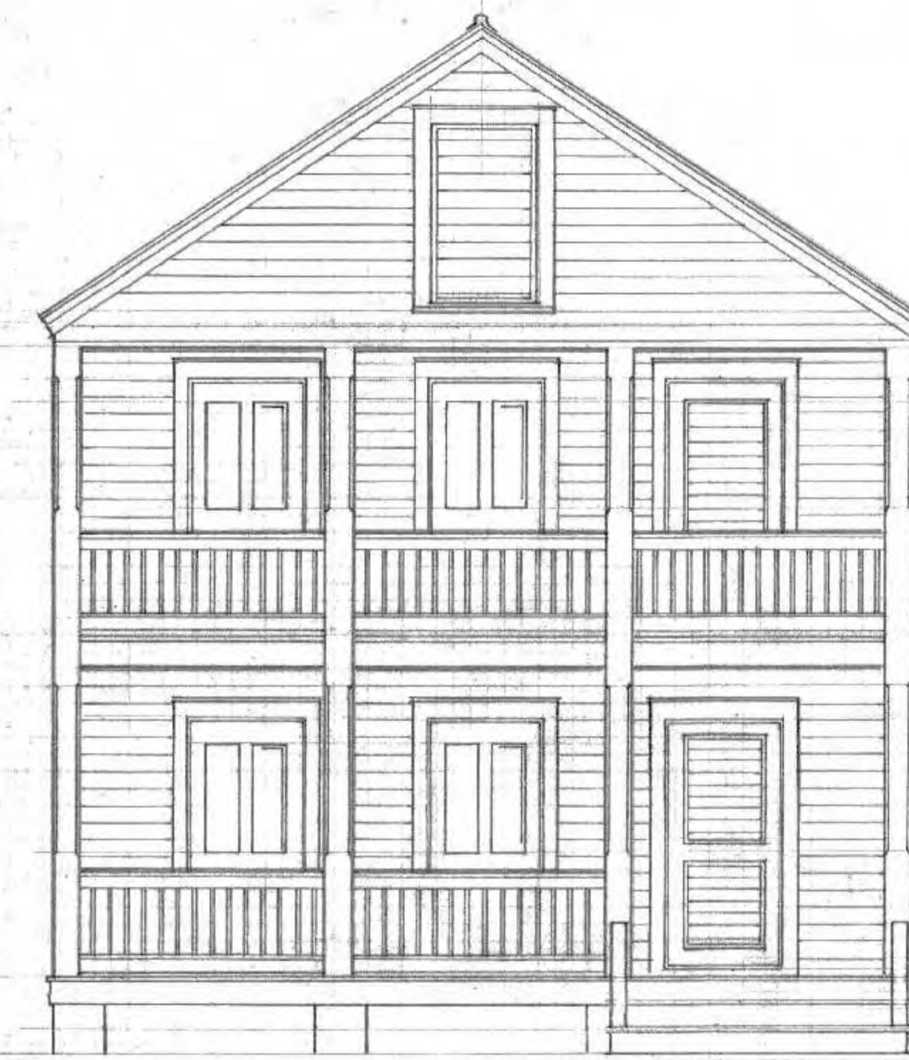
NORTHWEST ELEVATION 1/4"=1'-0"
