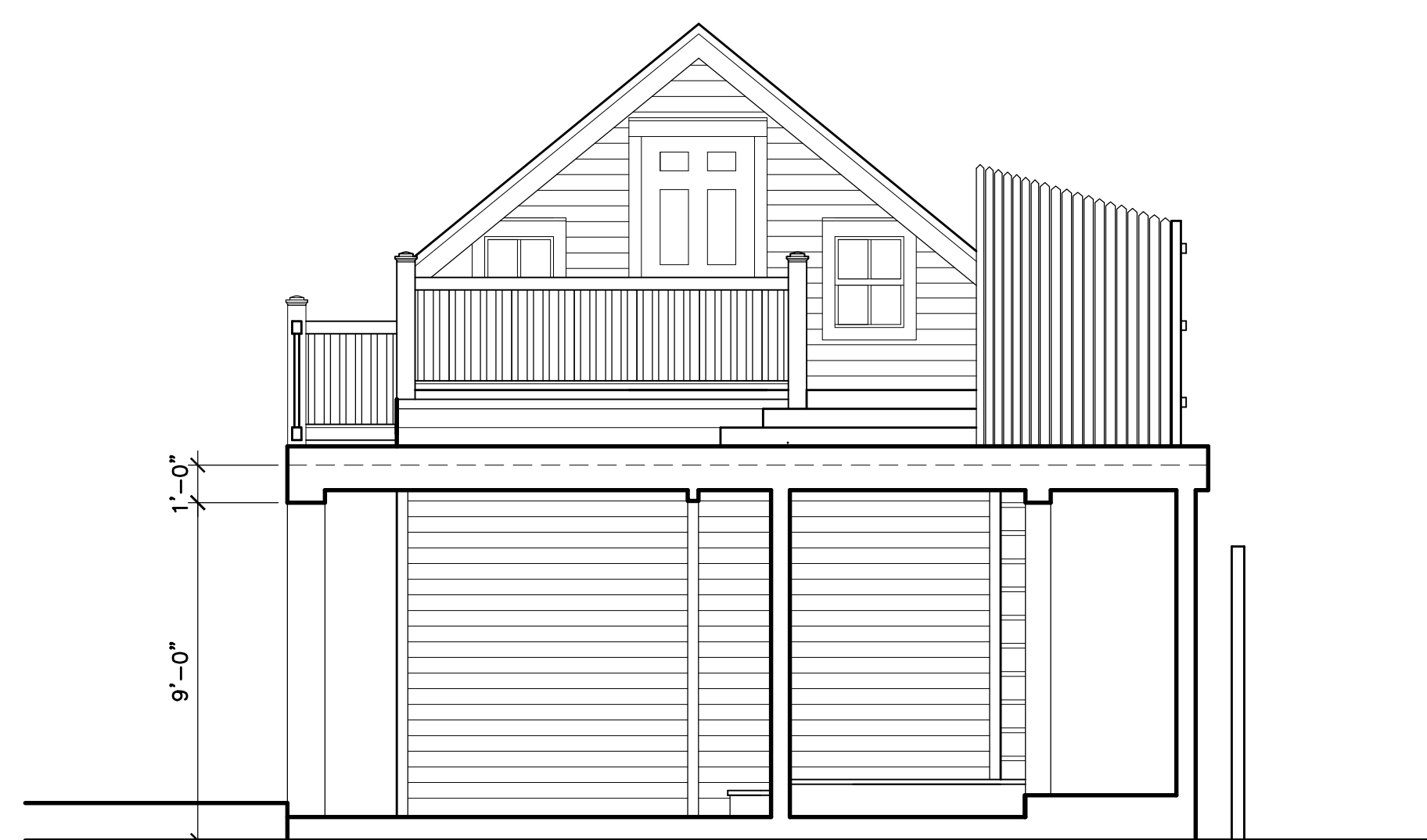
B EX-3 EXISTING REAR ELEVATION SCALE: 1/4"=1'-0"
