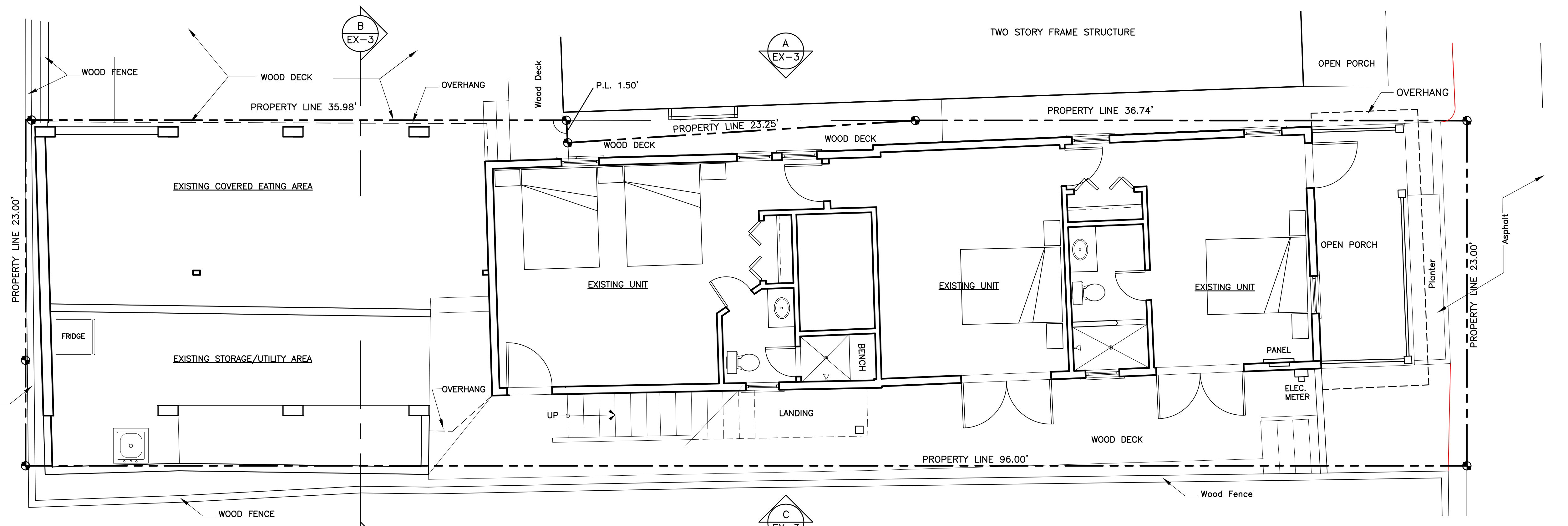
EXISTING FIRST FLOOR PLAN SCALE: 1/4"=1'-0"
