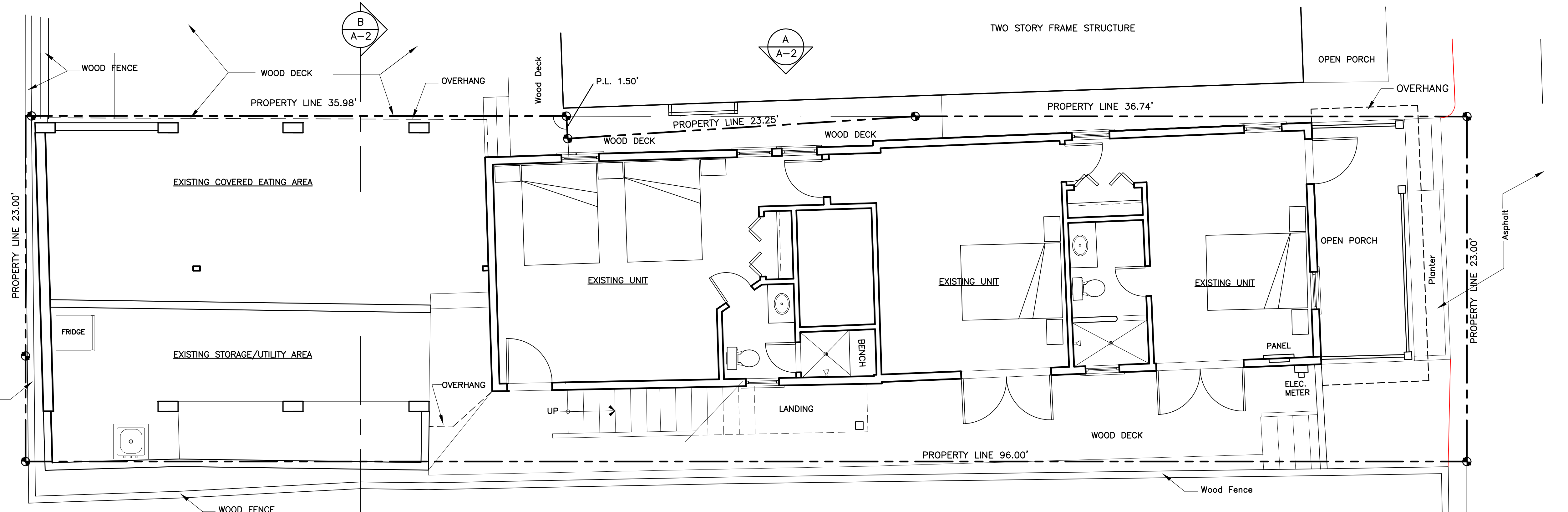
REVISED FIRST FLOOR PLAN
