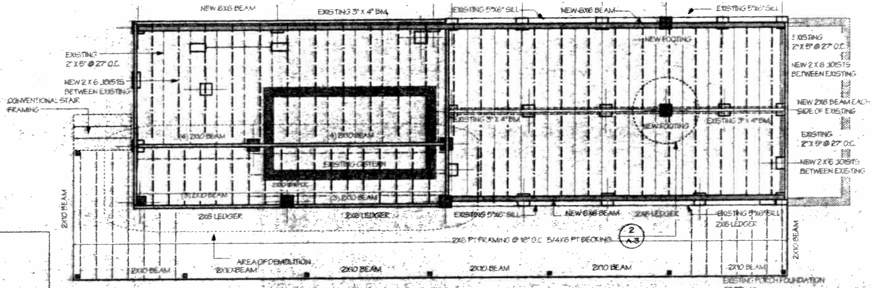
1st FLOOR FRAMING PLAN SCALE: 1/4" = 1'-0"
