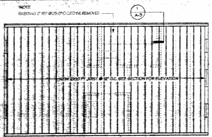
2 FLOOR FRAMING PLAN SCALE: 1/4" = 1'-0"
