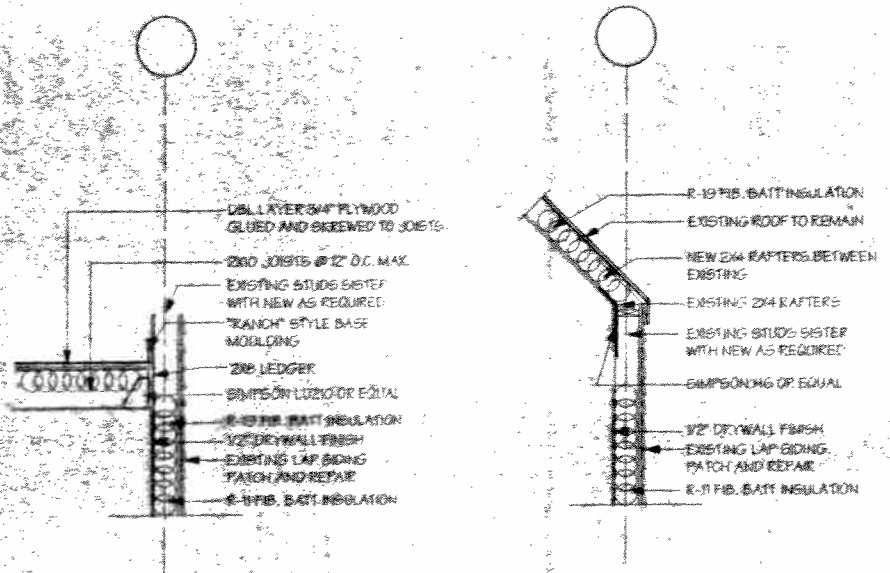
1 WALL/FLOOR CONNECTION DETAIL SCALE: 1/2" = 1'-0" 3 WALL/ROOF CONNECTION DETAIL SCALE: 1/2" = 1'-0"
