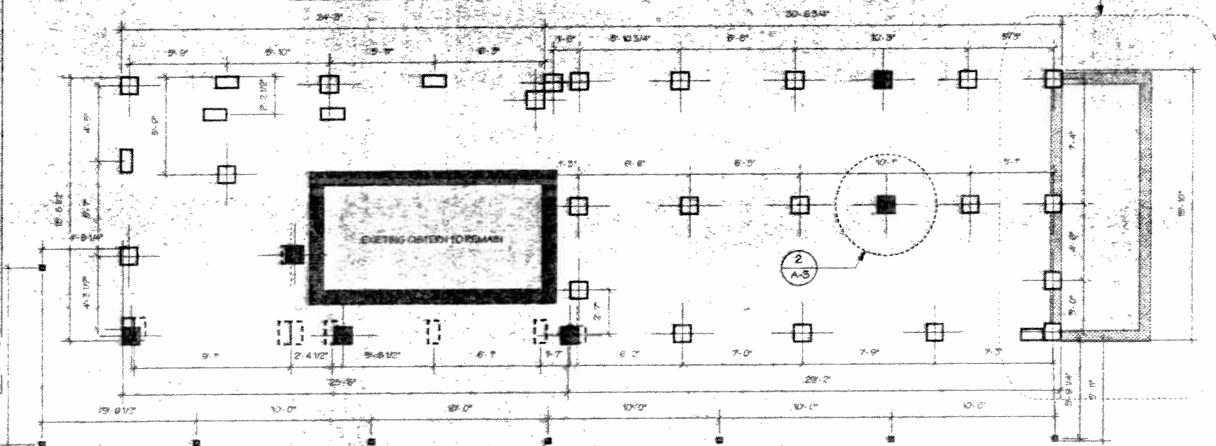
1st FLOOR FOUNDATION PLAN SCALE: 1/4" = 1'-0"
