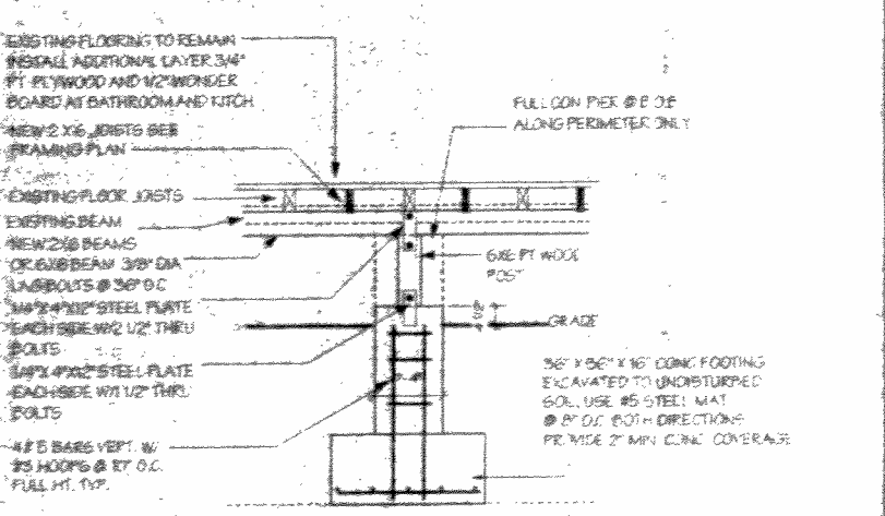
2 TYPICAL FOOTING & COL. DETAIL SCALE: 1/2" = 1'-0"
