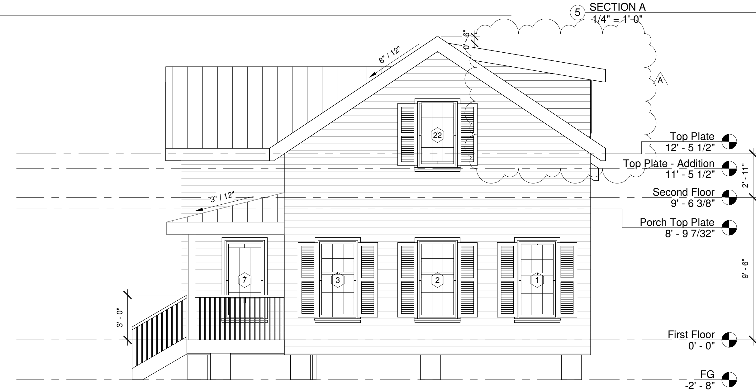
④ South 1/4" = 1'-0"
