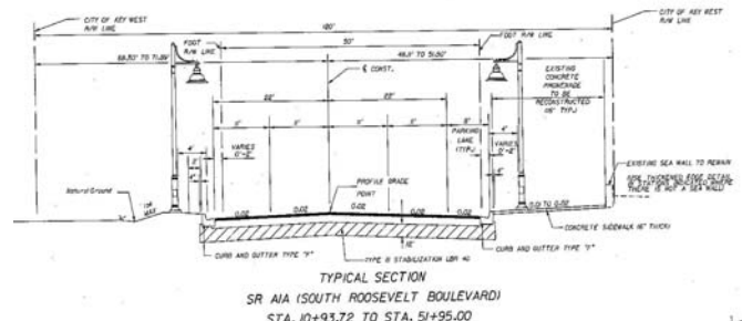
Current proposed cross section at parking area/La Brisa
