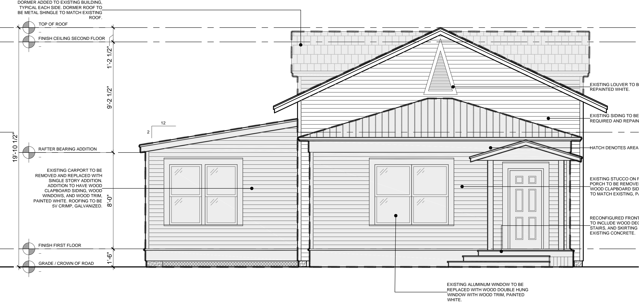
01 East Elevation - Margaret Street 1/4" = 1'-0"
