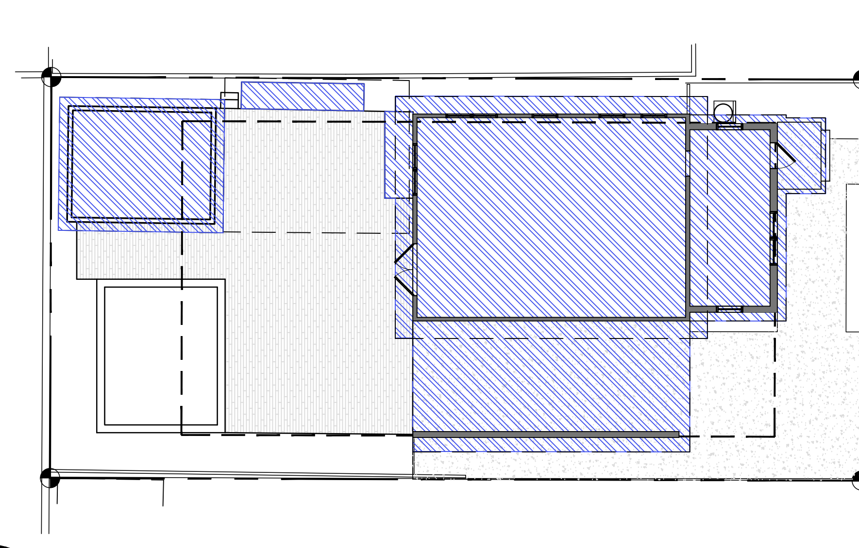
02 Building Coverage Plan - Existing 1,996 Square Feet (47%) 3/32" = 1'-0"
