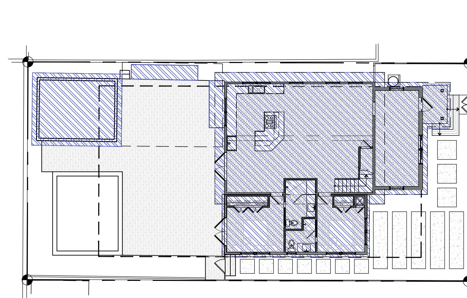
01 Building Coverage Plan - Proposed 1,933 Square Feet (45%) 3/32" = 1'-0"
