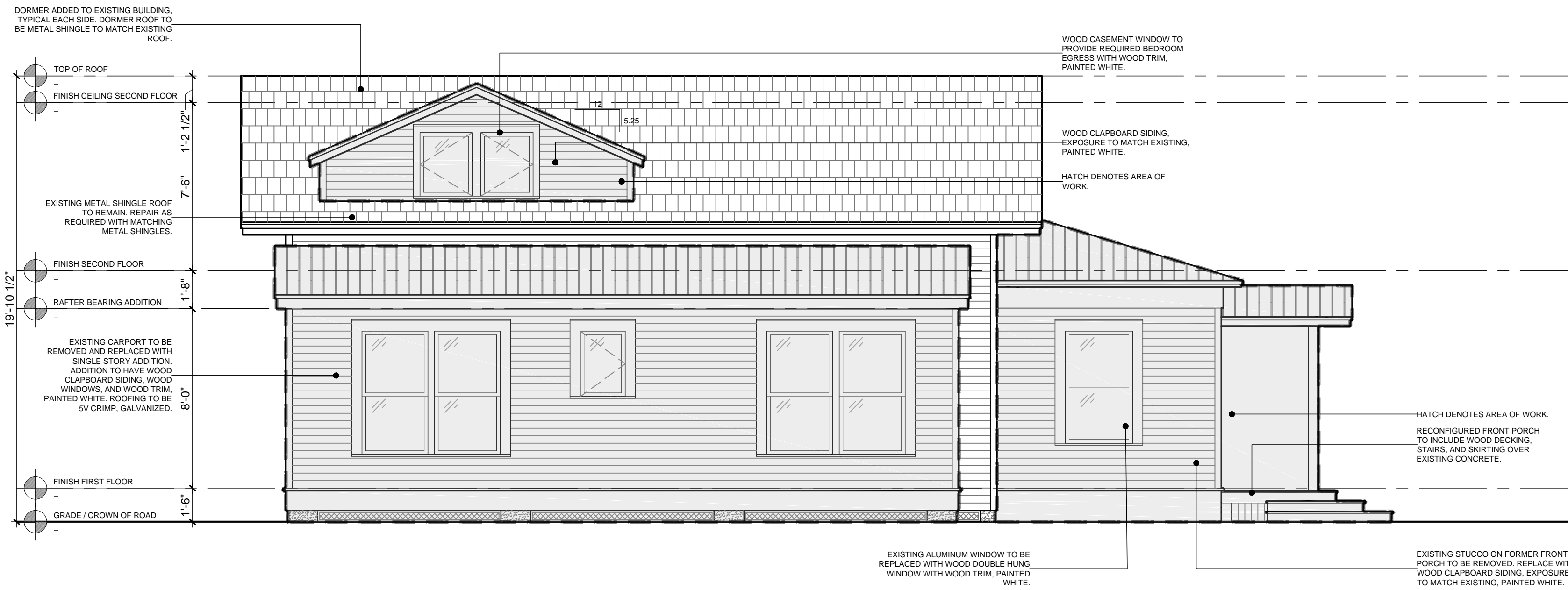
04 South Elevation 1/4" = 1'-0"
