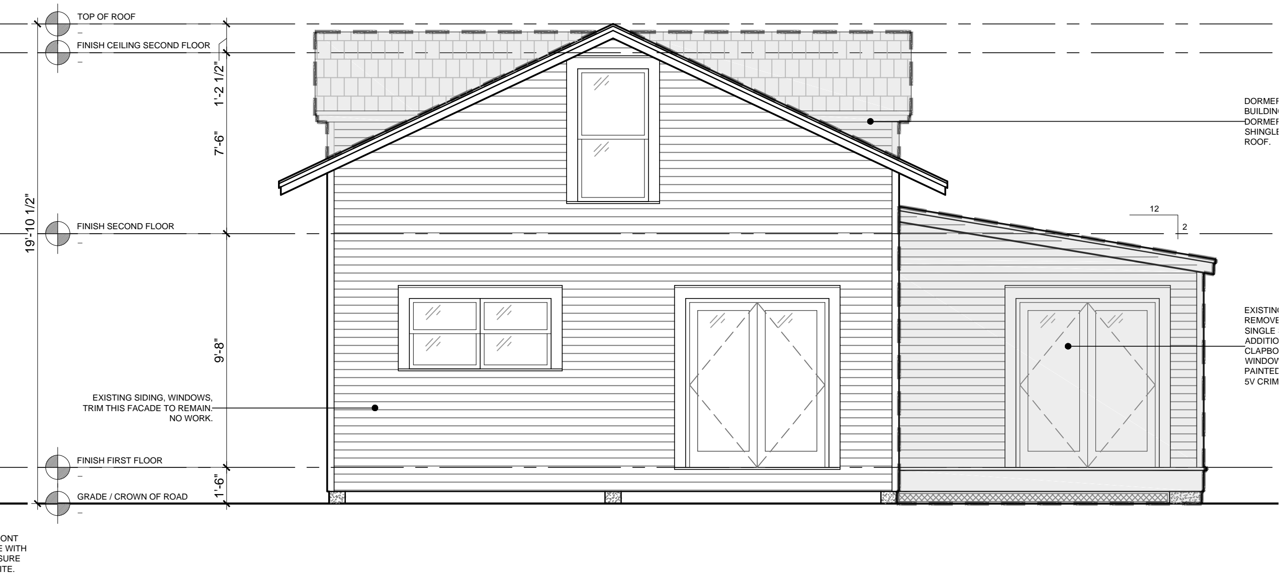
03 West Elevation 1/4" = 1'-0"
