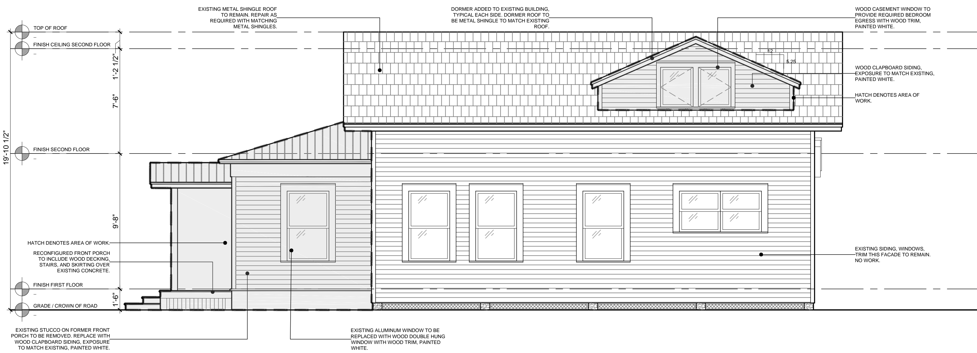
02 North Elevation 1/4" = 1'-0"
