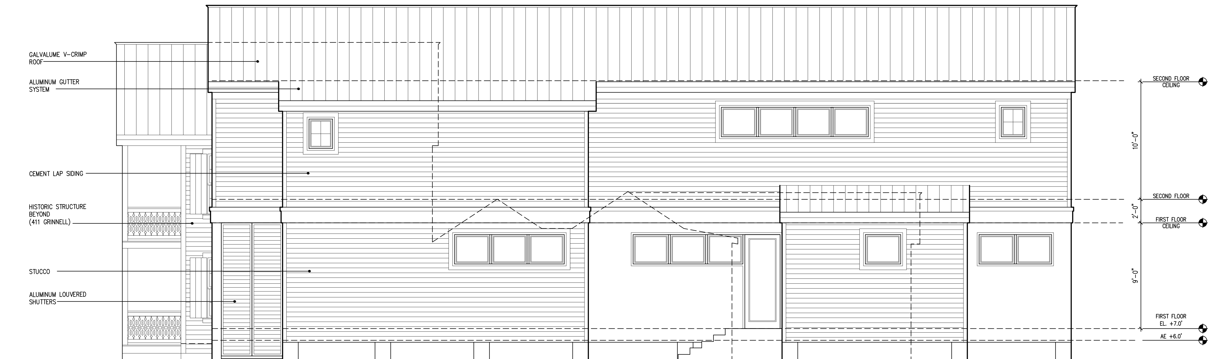
SIDE ELEVATION (SOUTH) 1/4"=1'-0"
