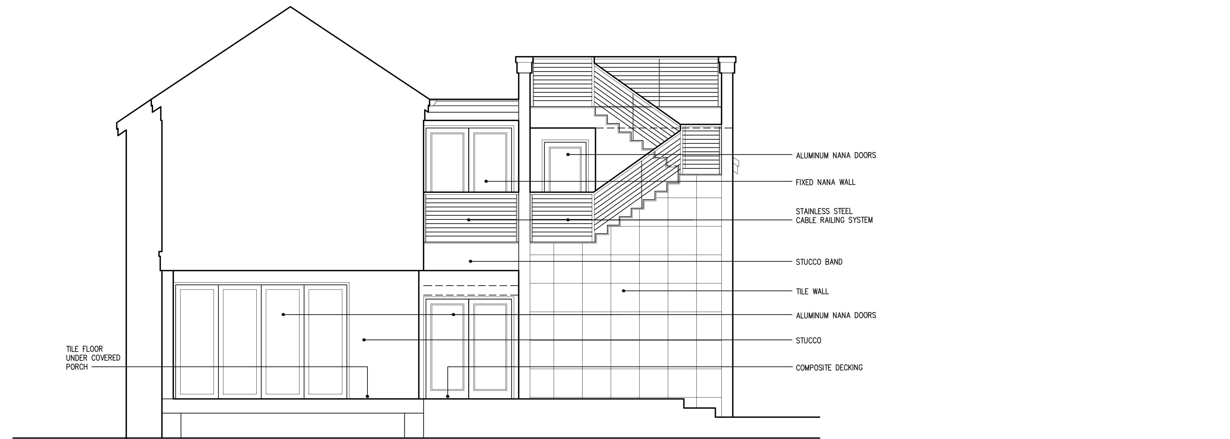
PARTIAL REAR ELEVATION (EAST) 1/4"=1'-0"
