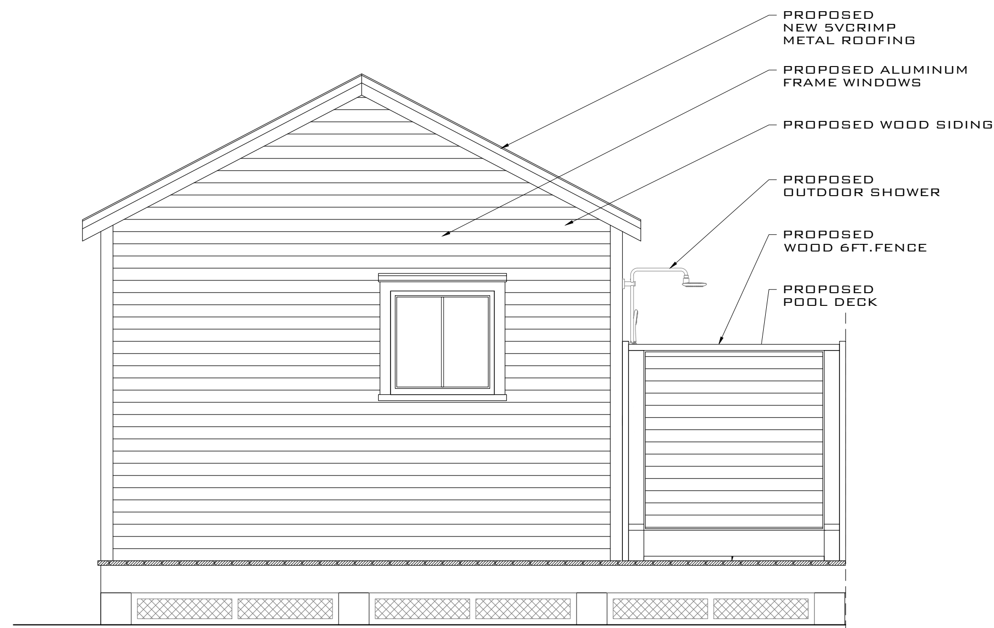
PROPOSED LEFT ELEVATION (POOL HOUSE) SCALE: 3/8" = 1'-0"
