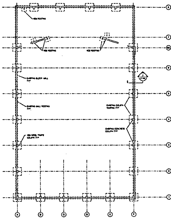
EXISTING FOUNDATION PLAN
