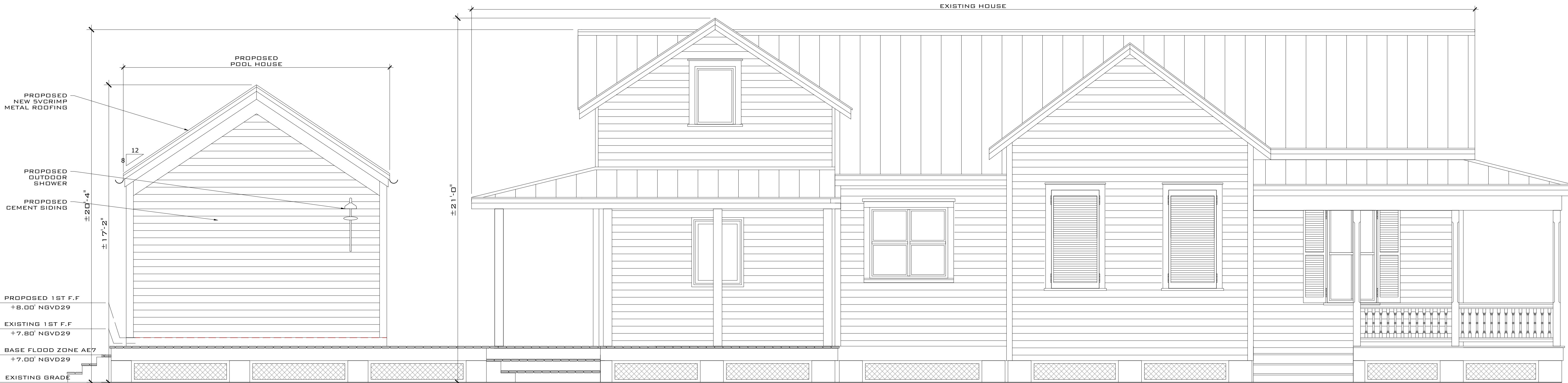
PROPOSED LEFT ELEVATION SCALE: 3/8" = 1'-0"
