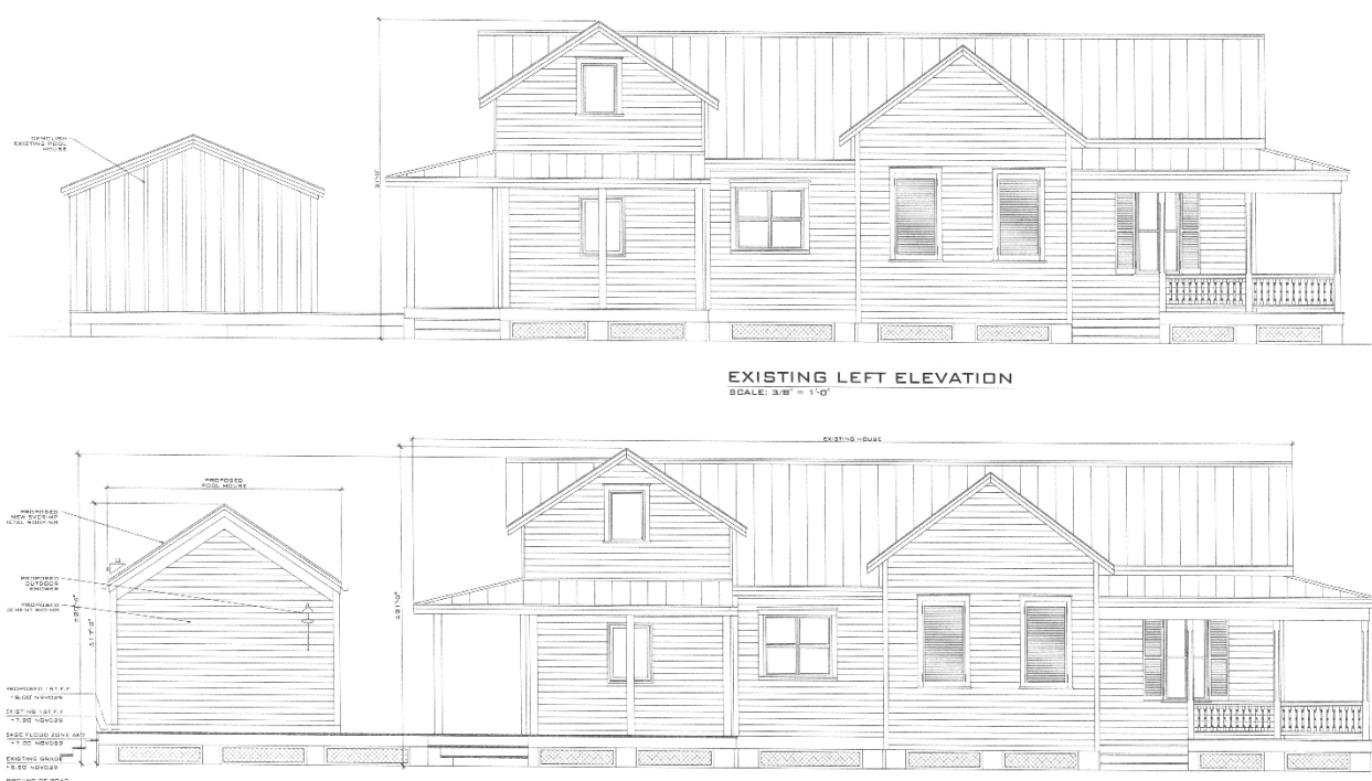
Current and proposed south elevation.
