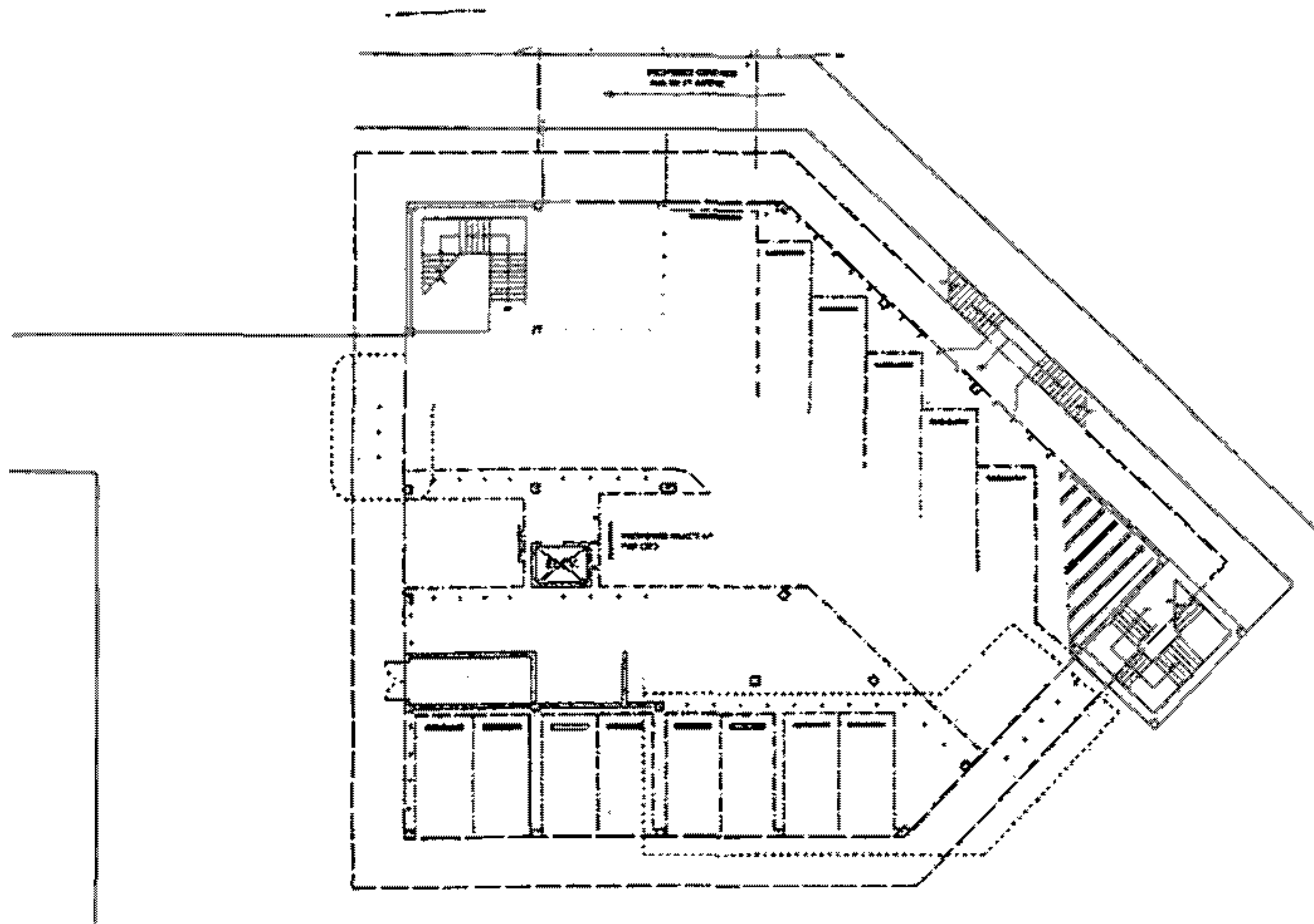
EXHIBIT A-1 YANKEE FREEDOM STORAGE FIRST FLOOR KEY WEST BIGHT FERRY TERMINAL
