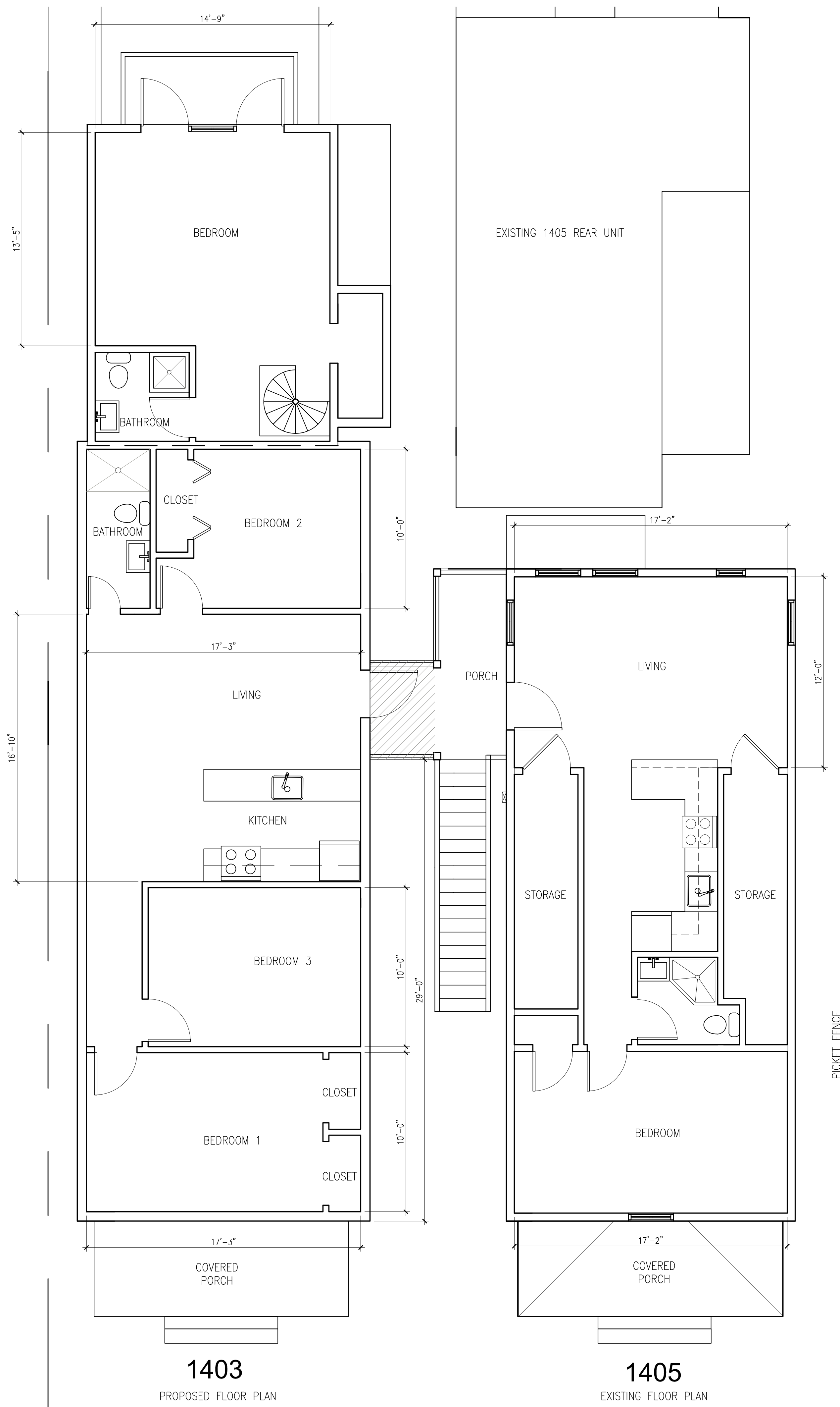
3 SECOND FLOOR PLANS 1403-1405 SCALE: 1/4"=1'-0"
