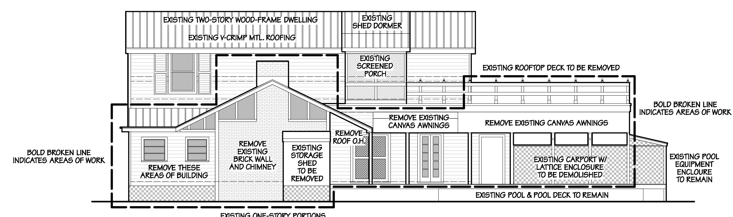
EXISTING WEST ELEVATION scale: 1/8"=1'-0"
