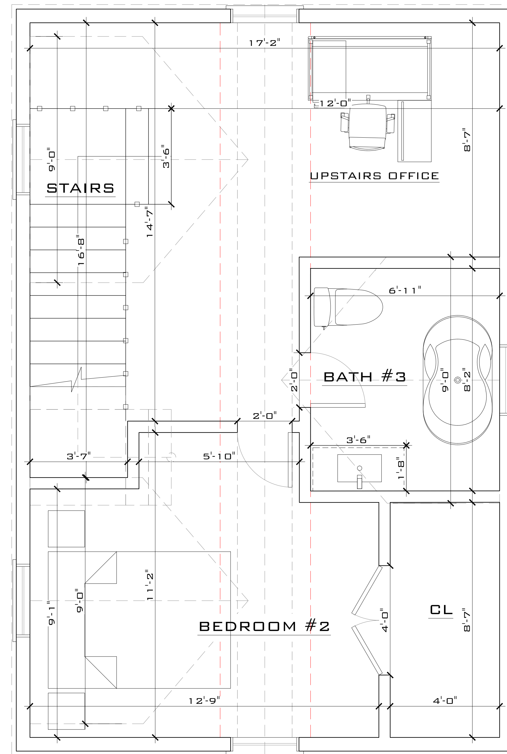
PROPOSED 2ND FLOOR PLAN SCALE: 1/4" = 1'-0"
