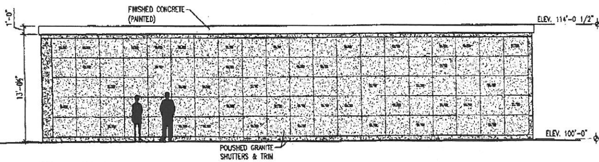
Ⓐ FRONT ELEVATION
