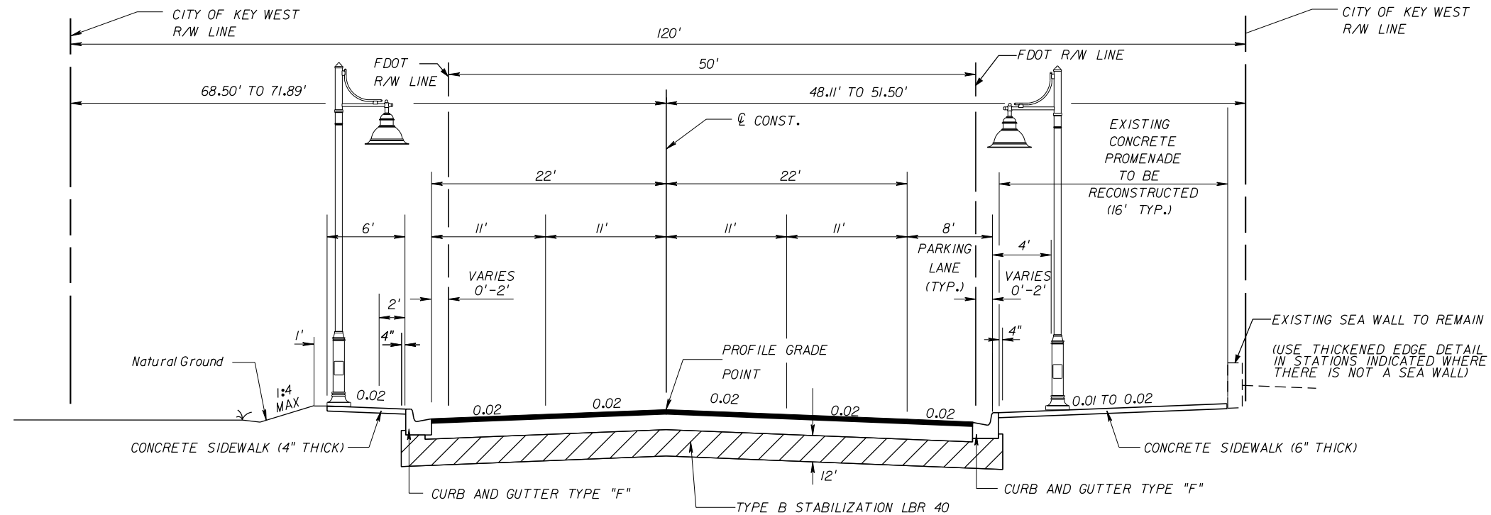
TYPICAL SECTION SR AIA (SOUTH ROOSEVELT BOULEVARD) STA. 10+93.72 TO STA. 51+95.00
