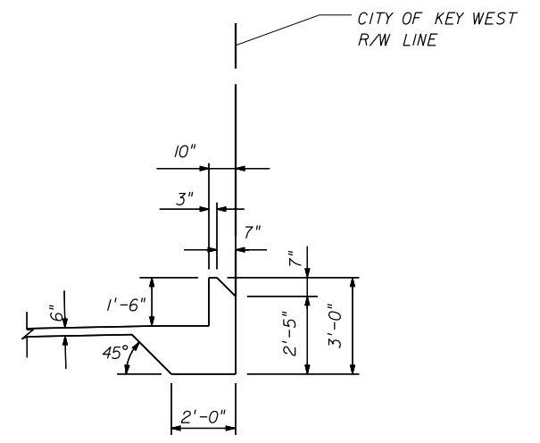
STD. THICKENED EDGE AND PARAPET WALL DETAIL
