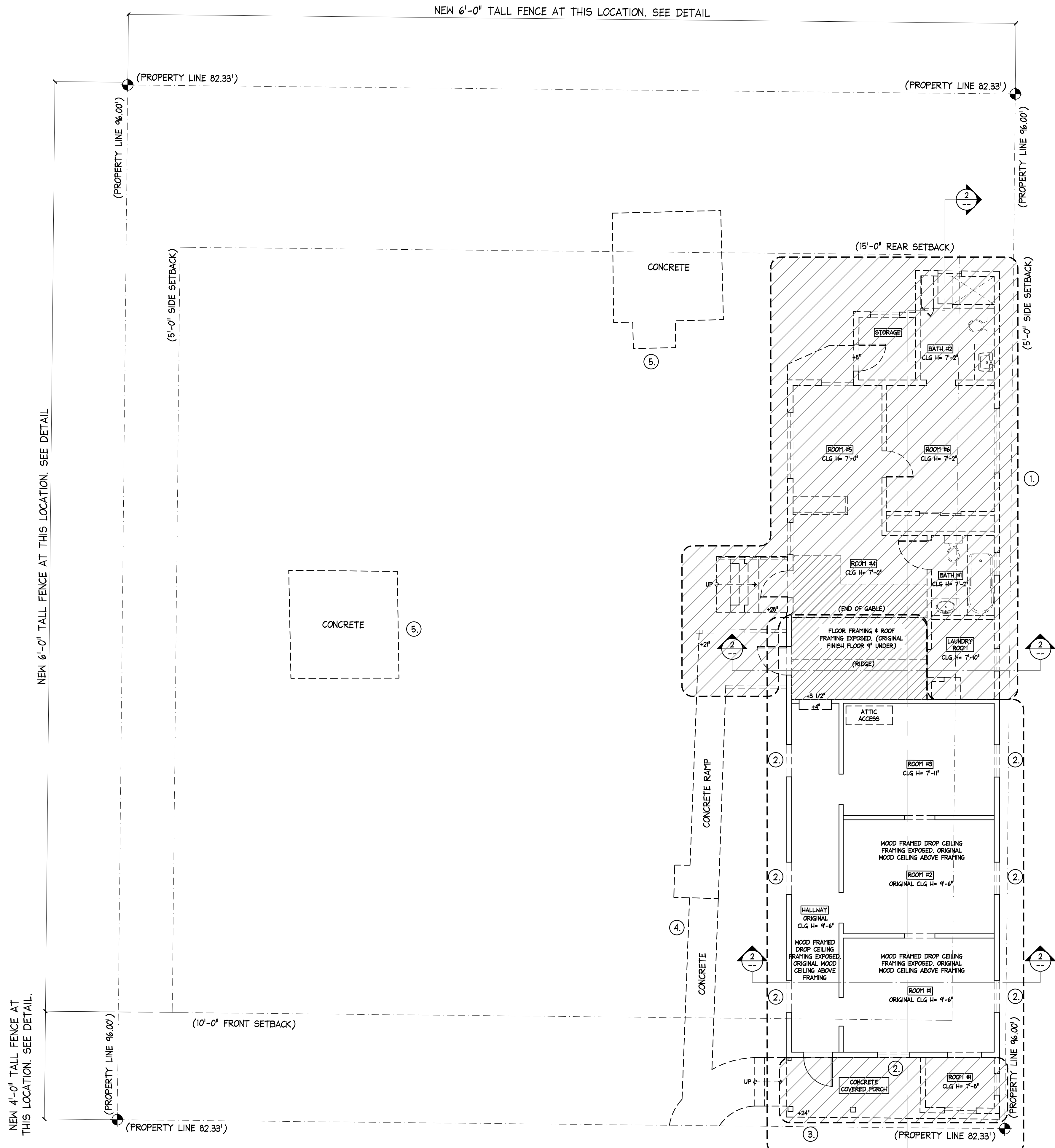
1 A2 EXISTING SITE PLAN SCALE: 3/16" = 1'-0"
