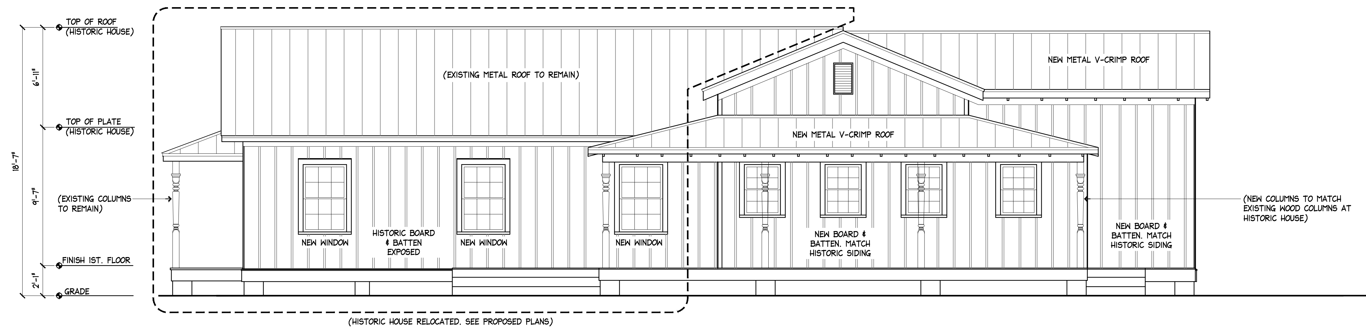
1 PROPOSED SOUTH ELEVATION SCALE: 1/4" = 1'-0"
