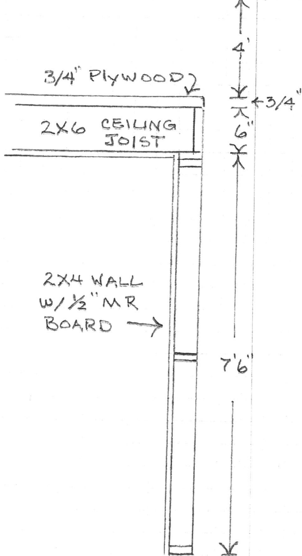
BATHROOM WALL ELEVATION
