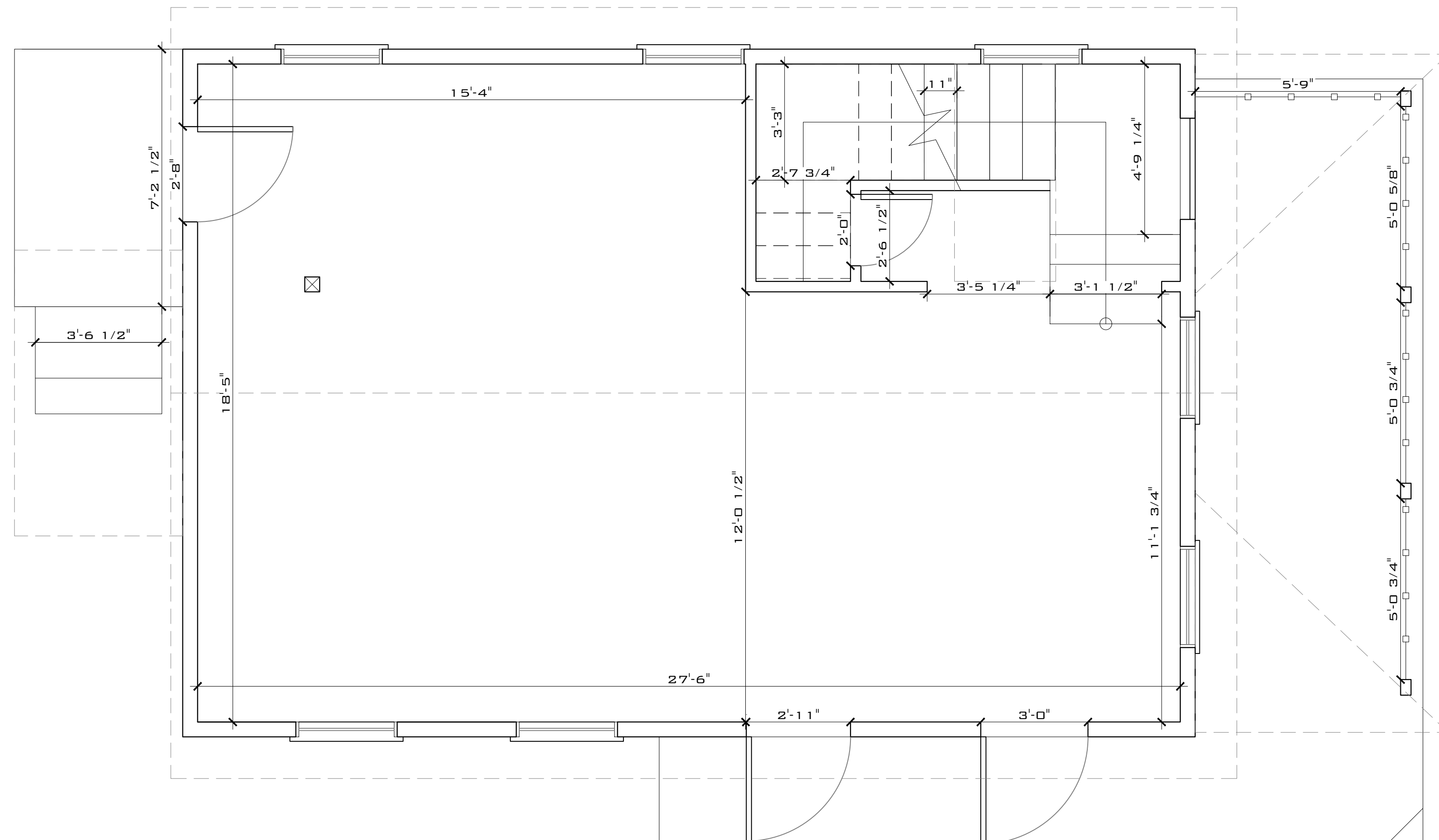
EXISTING 1ST FLOOR PLAN
