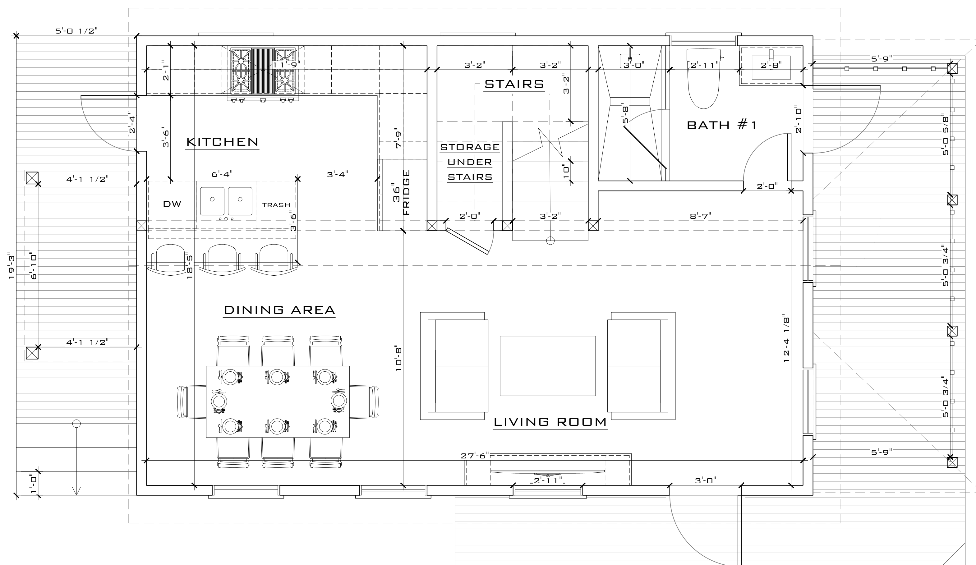
PROPOSED 1ST FLOOR PLAN
