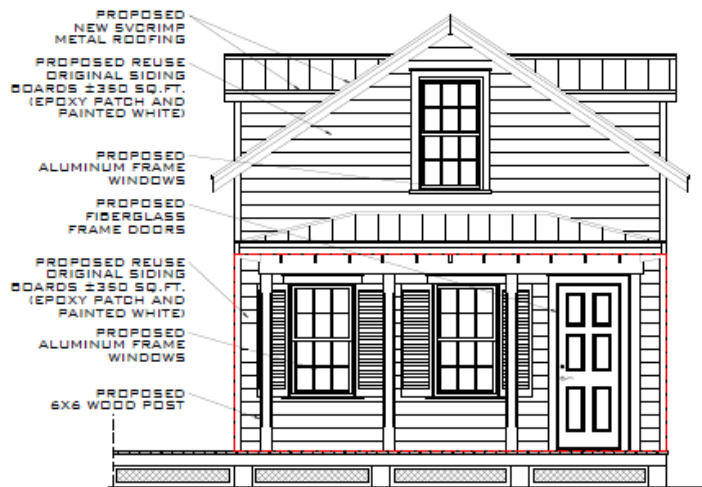
PROPOSED RIGHT ELEVATION SCALE: 3/8" = 1'-0"
