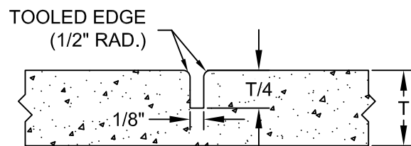
CONTRACTION JOINT
