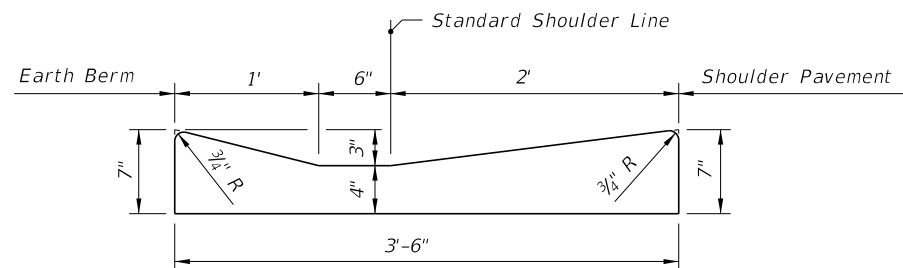
SHOULDER GUTTER
