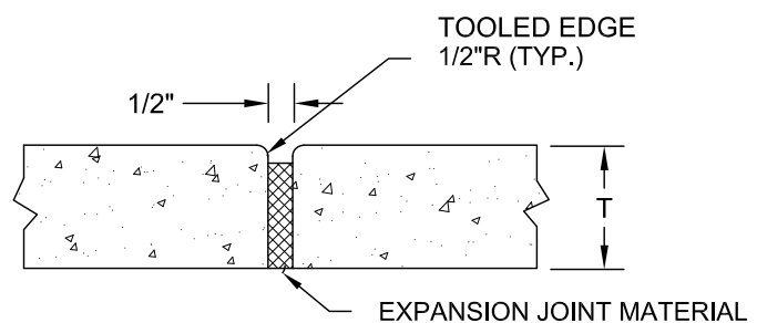
EXPANSION JOINT
