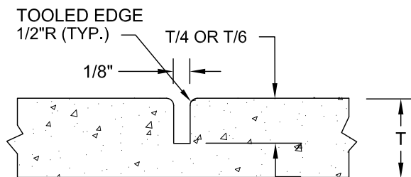
TYPICAL SIDEWALK SECTION
