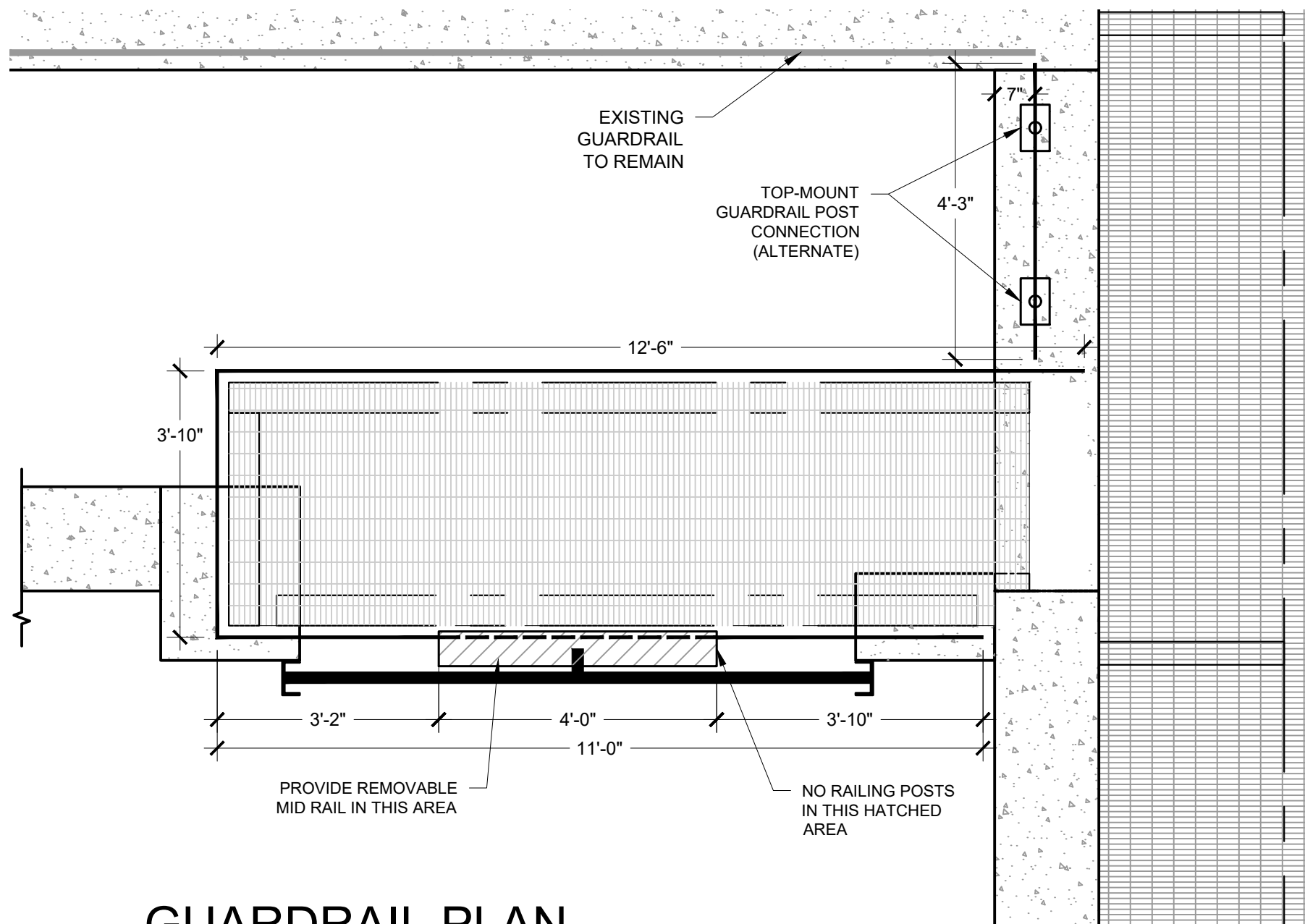
GUARDRAIL PLAN
