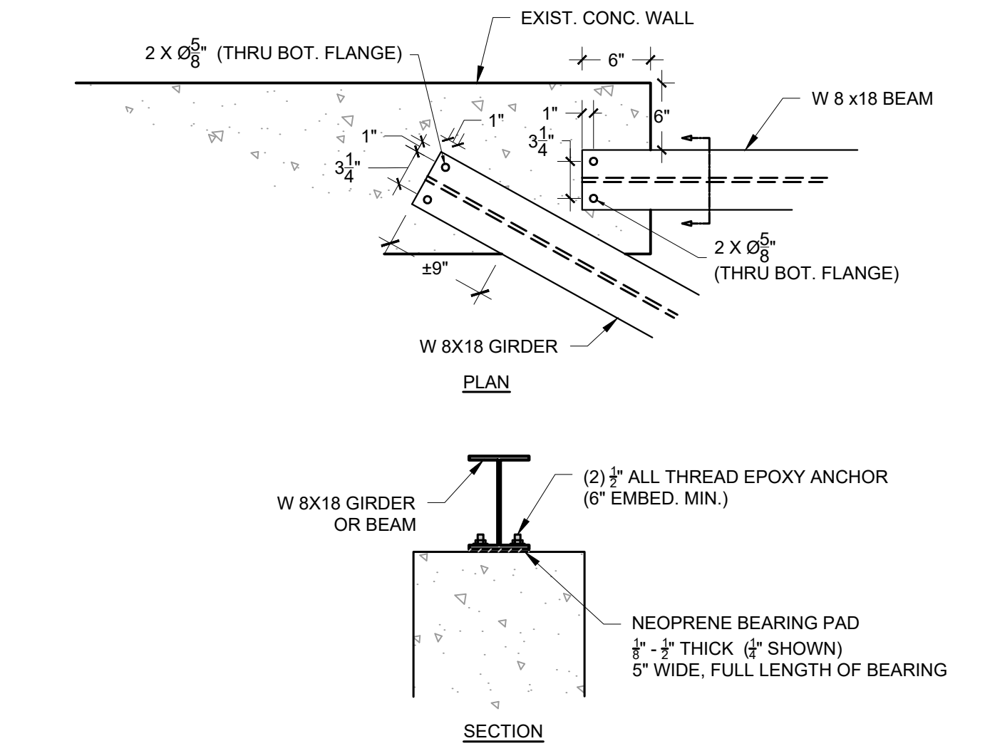
1 S-5 DETAIL - GIRDER BEARING ON WALL SCALE: 1"=1'-0"
