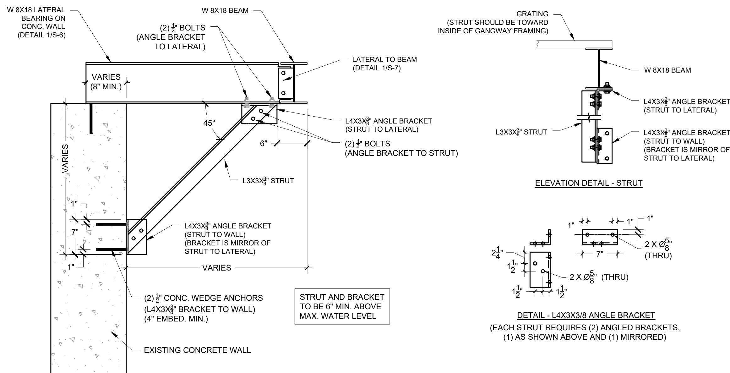
2 TYP. DETAIL - LATERAL CONNECTION
