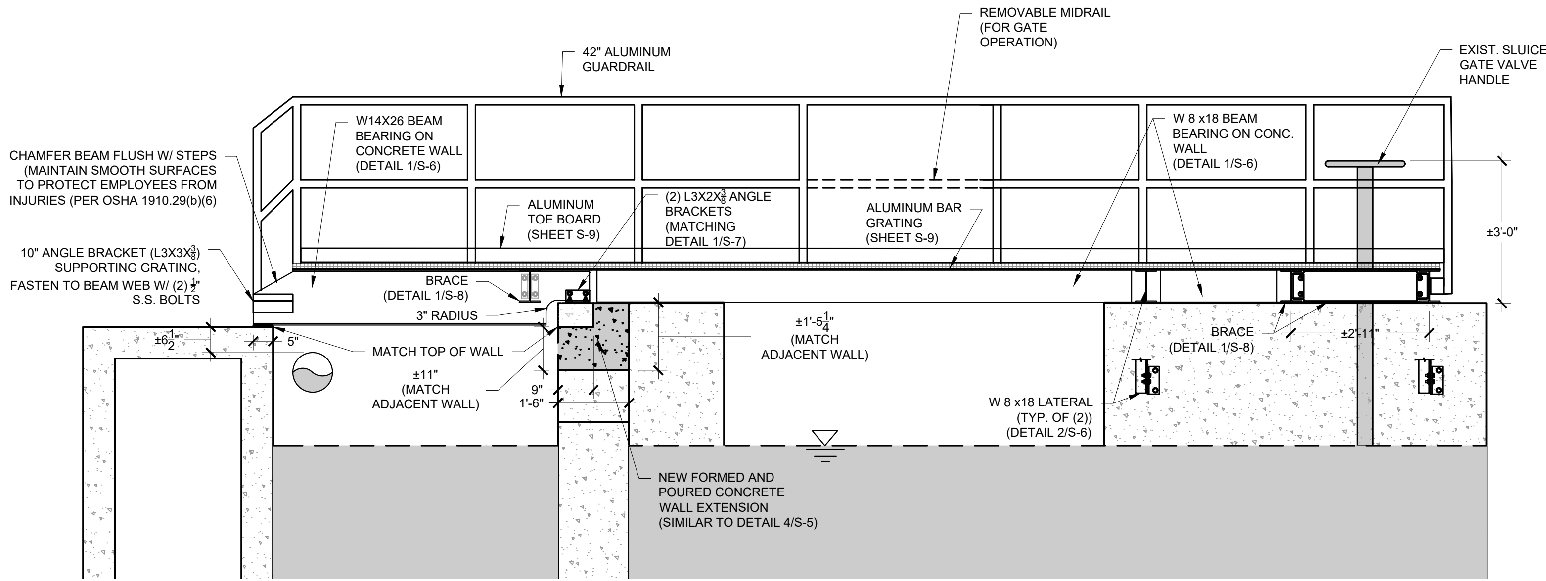
A S-8 SECTION - GANGWAY 4 PROPOSED SCALE:1/2"=1'-0"
