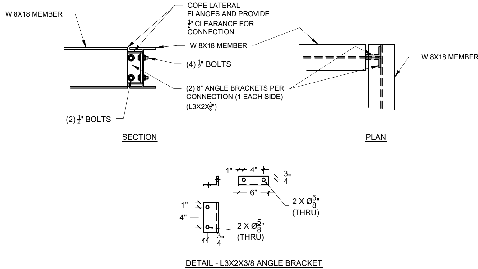
1 S-7 TYP. DETAIL - CONNECTION BETWEEN W SECTIONS
