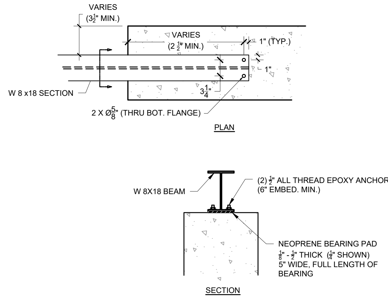
1 TYP. DETAIL - BEAM BEARING ON WALL
