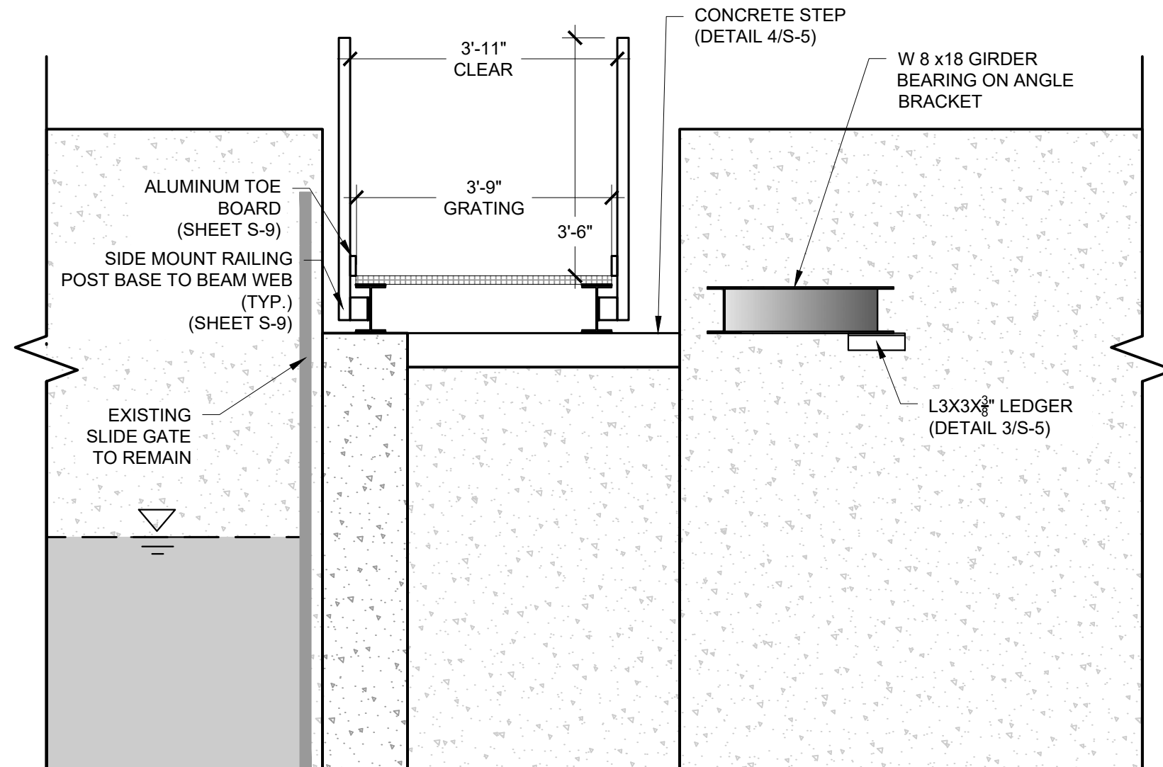
B S-5 SECTION - GANGWAY 1 PROPOSED SCALE: 1/2"=1'-0"
