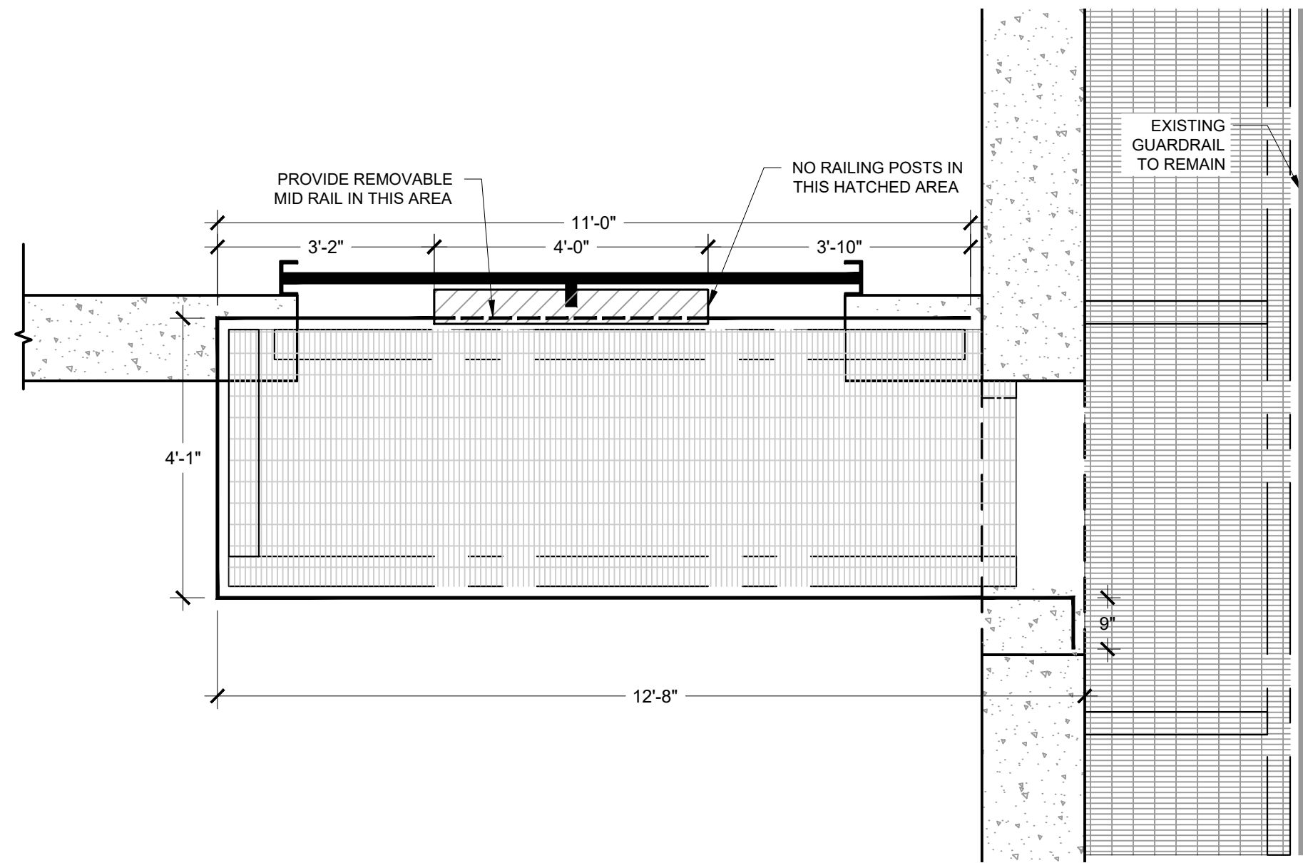
GUARDRAIL PLAN
