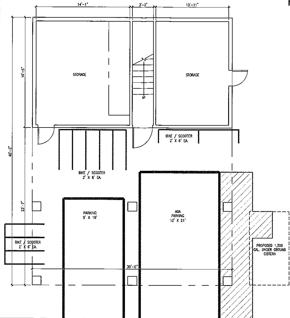
3 A2.1 GROUND LEVEL PLAN SCALE: 1/4"=1'-0"
