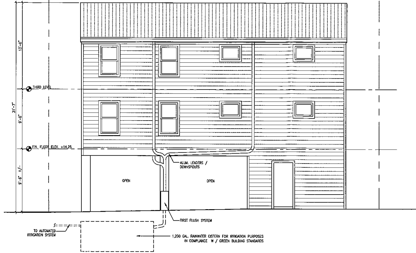
2 WEST ELEVATION SCALE: 1/4"=1'-0"
