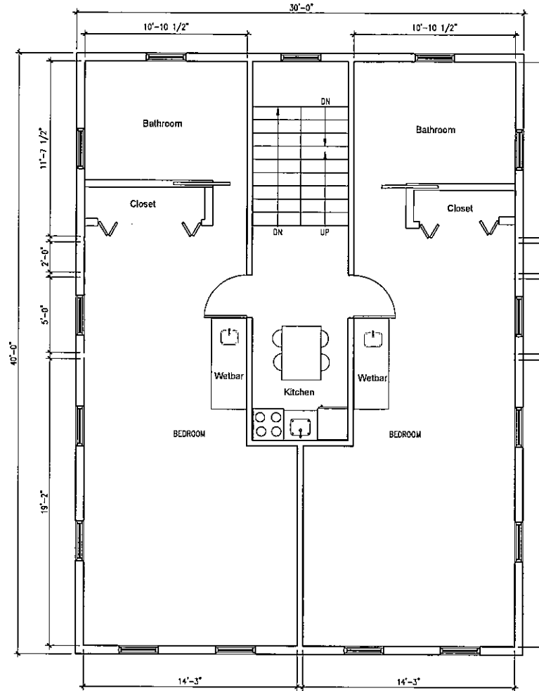
4 A2.1 SECOND LEVEL PLAN SCALE: 1/4"=1'-0"
