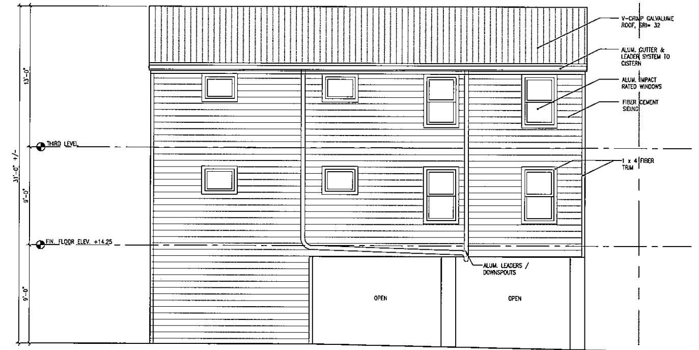
4 EAST ELEVATION SCALE: 1/4"=1'-0"
