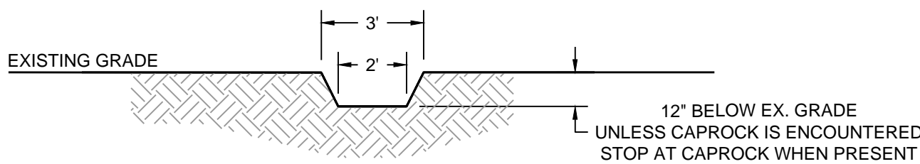
FLUSHING CUT CROSS SECTION - TYPICAL SCALE: N.T.S.
